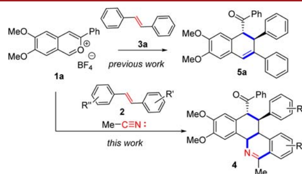
Figure 2. New one-step synthesis of benzo[ c ]phenanthridines.
