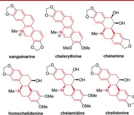
Figure 1. Representative bioactive benzo[ c ]phenanthridine derivatives.
