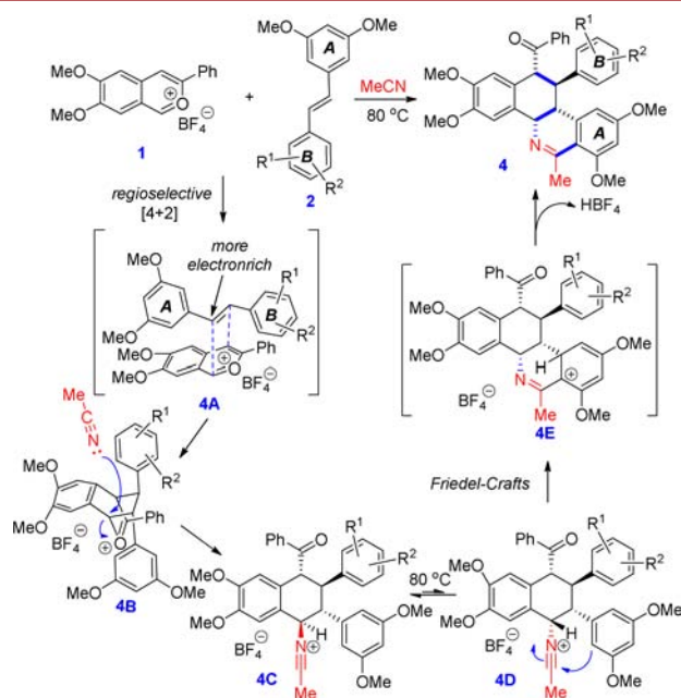
Figure 3. Proposed mechanism for the multistep cascade reaction.
