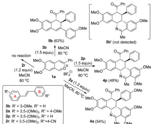
Scheme 1. Examination of the Reactions of ICTB 1a with Stilbenes 2a,p,r and 3b
